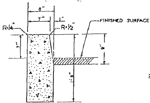
TYPE "A"
