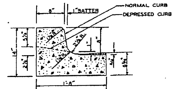
INTERGRAL R.C.C. CURB & GUTTER TYPE "3"
