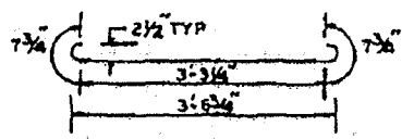
BAR "B" 5/8" BARS 3'-6 3/4" LONG
