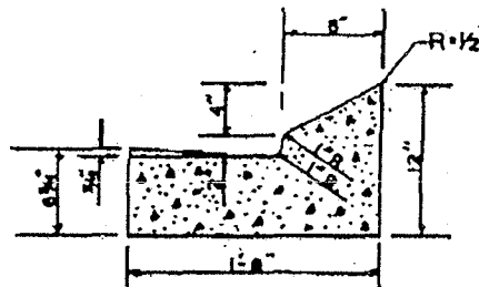
R.C.C. PARKWAY CURB TYPE "3"
