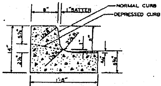
INTERGRAL R.C.C. CURB & GUTTER TYPE "3"
