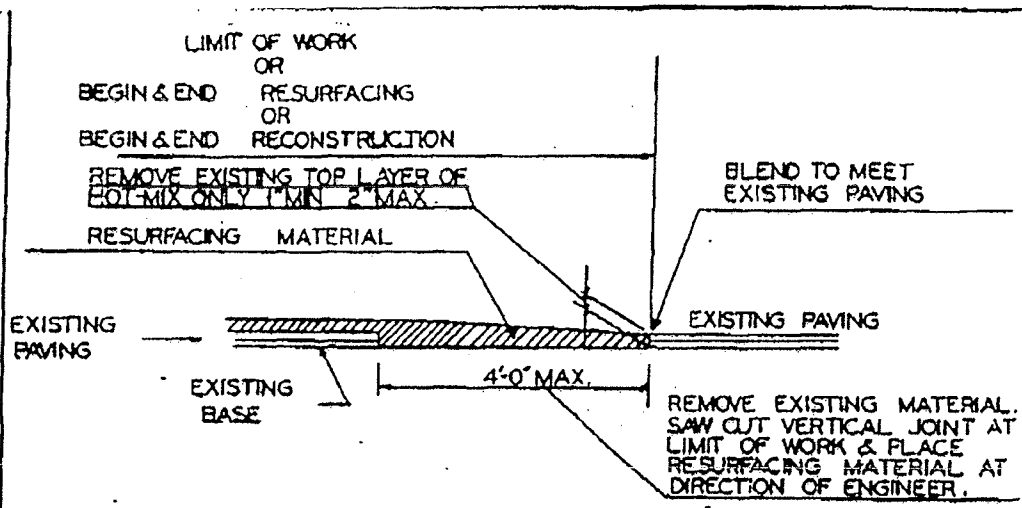
TYPICAL CUT JOINT DETAIL
